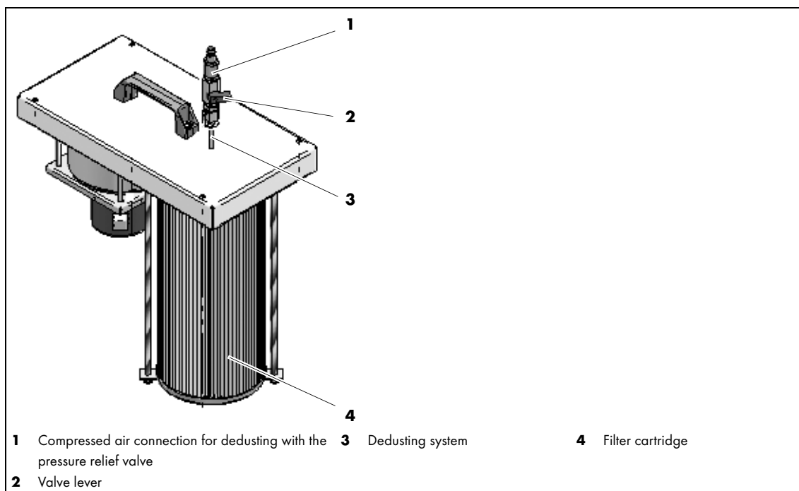
Fig. 3 Dedusting the fine filter cartridge
