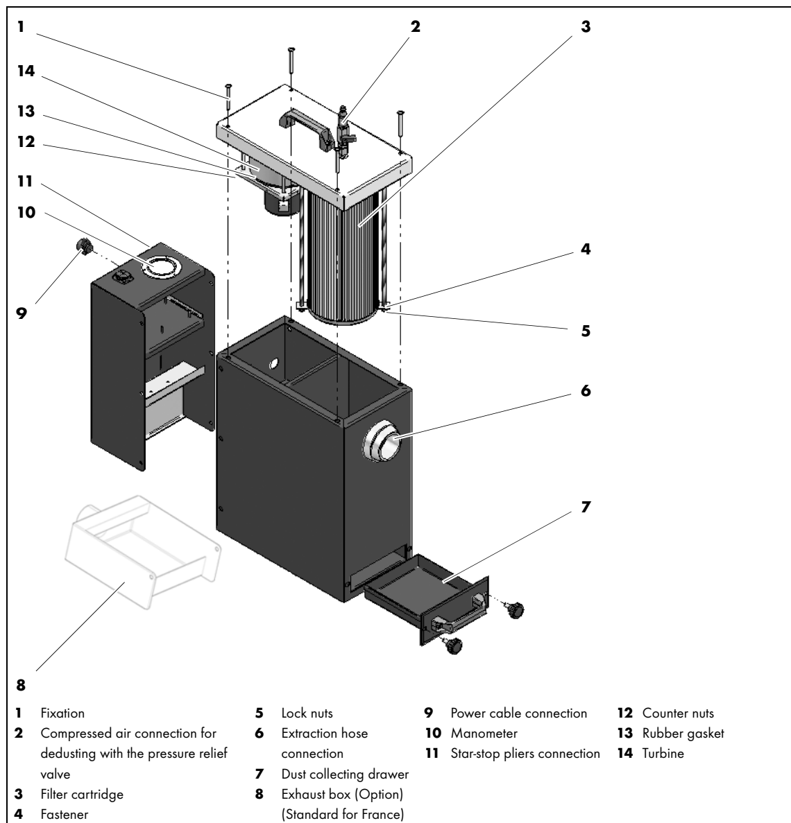
Fig. 2 Functional Description
