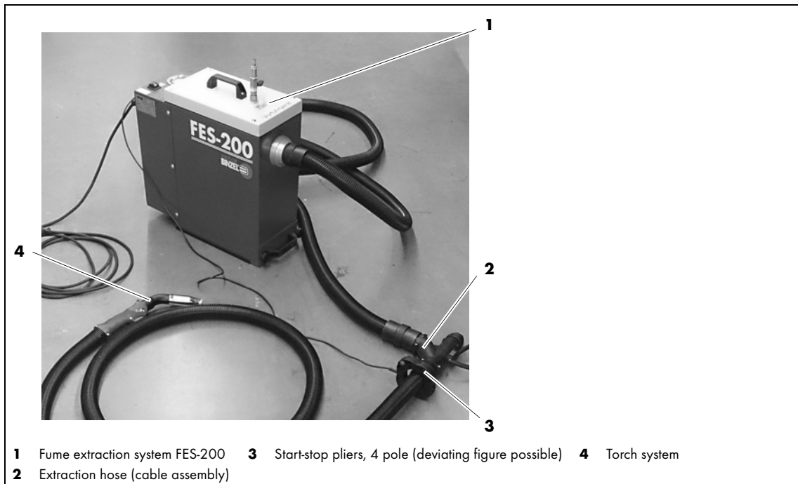
Fig. 4 Putting into operation
