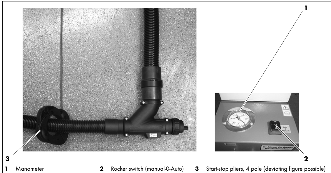
Fig. 5 Start-stop pliers
