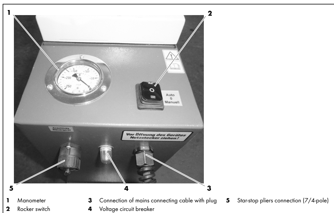
Fig. 6 Operating elements
